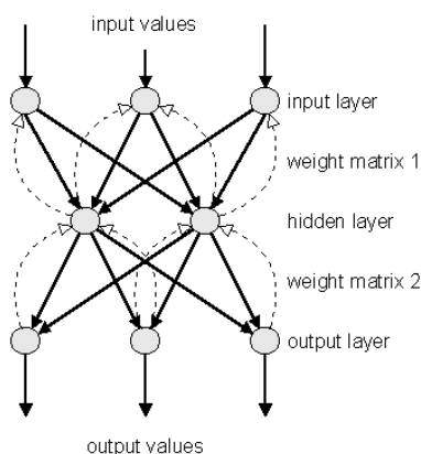
Figure 2 - A multilayer neural network with backpropagation error and one hidden layer
